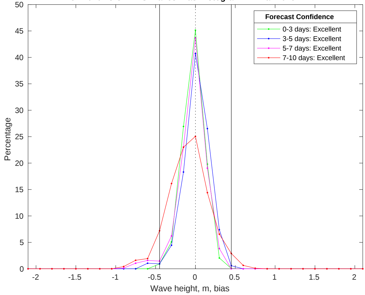
NDBC 41040 vs CMEMS Waves Bias Histogram: 11-Mar-2025
