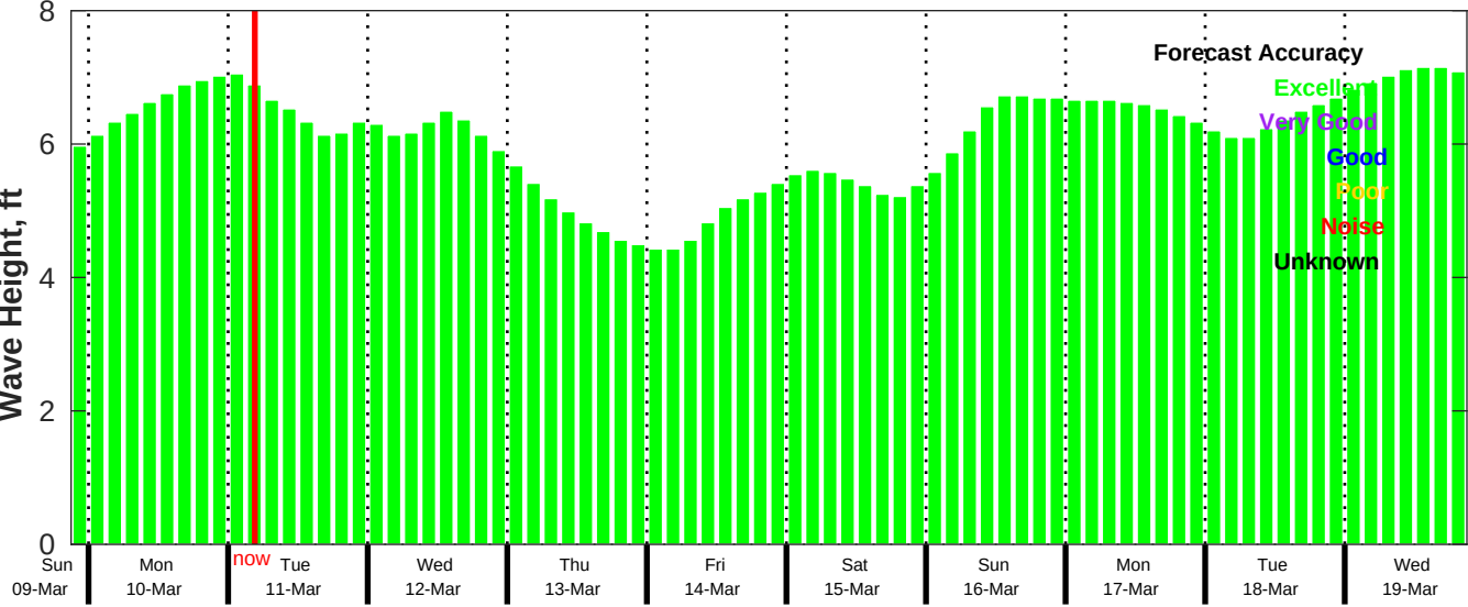
CMEMS Wave Forecast for NDBC 41040 from 09-Mar-2025 21:00:00 to 19-Mar-2025 21:00:00
