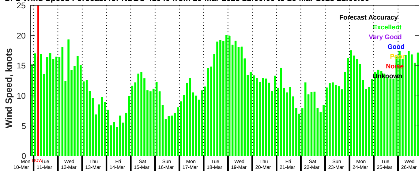
GFS Wind Speed Forecast for NDBC 41040 from 10-Mar-2025 21:00:00 to 26-Mar-2025 21:00:00
