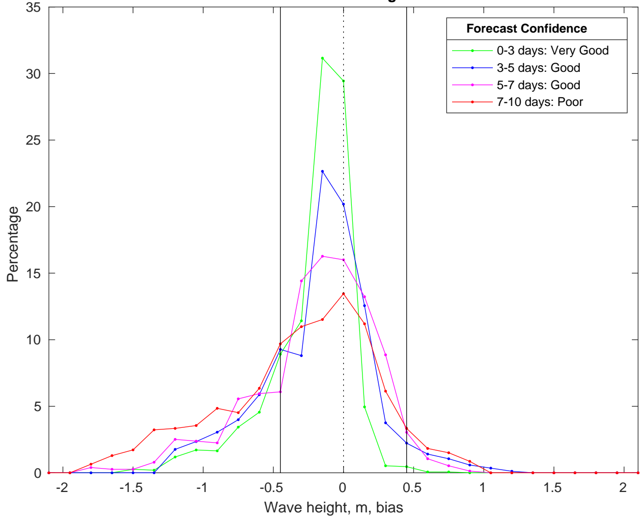
NDBC 42019 vs CMEMS Waves Bias Histogram: 11-Mar-2025
