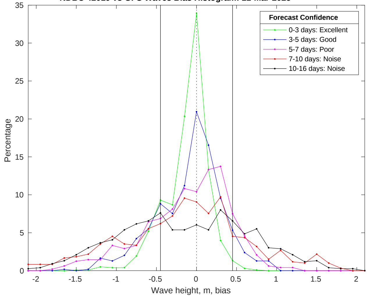
NDBC 42019 vs GFS Waves Bias Histogram: 11-Mar-2025
