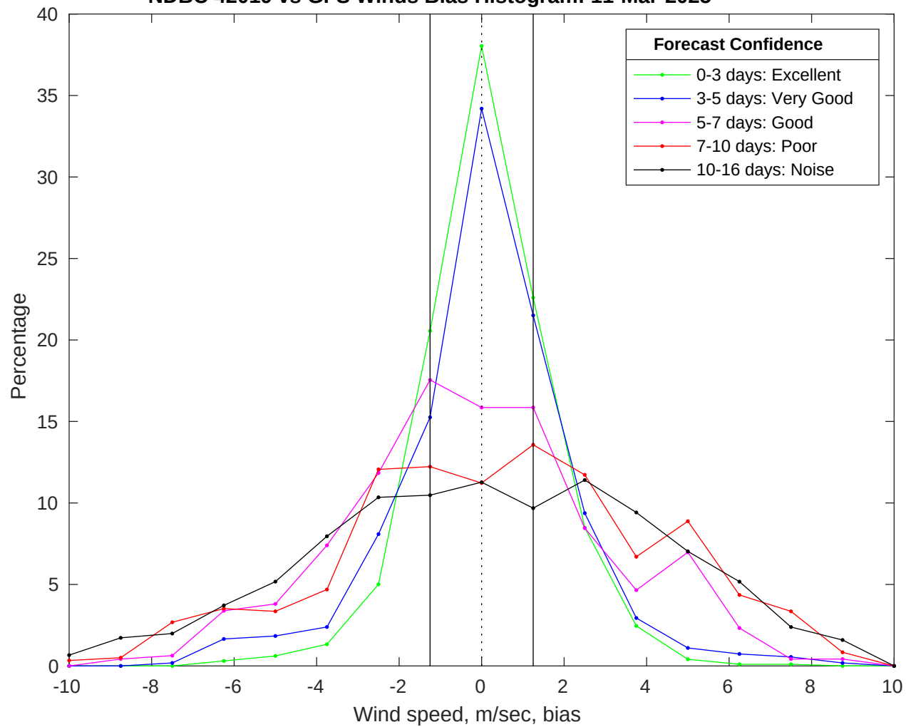
NDBC 42019 vs GFS Winds Bias Histogram: 11-Mar-2025
