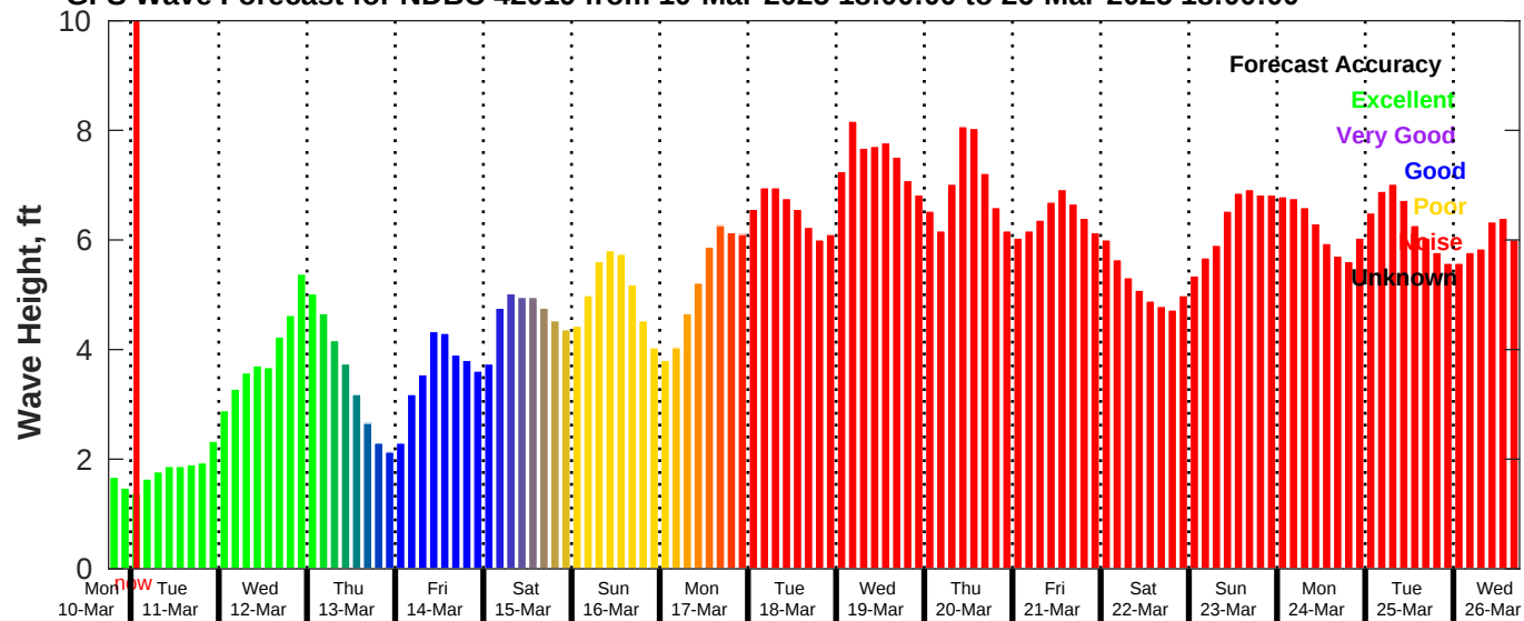
GFS Wave Forecast for NDBC 42019 from 10-Mar-2025 18:00:00 to 26-Mar-2025 18:00:00
