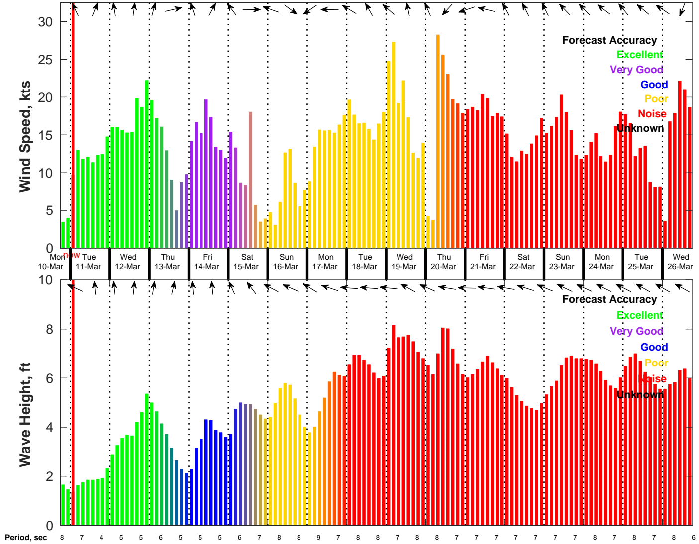
Wind & Wave Forecast for NDBC 42019 from 10-Mar-2025 18:00:00 to 26-Mar-2025 18:00:00
