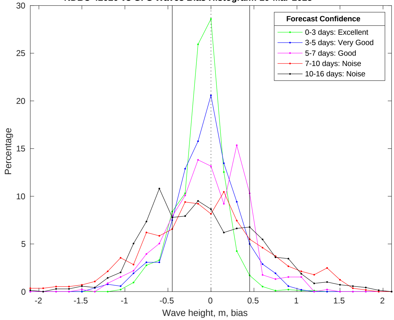
NDBC 42020 vs GFS Waves Bias Histogram: 10-Mar-2025
