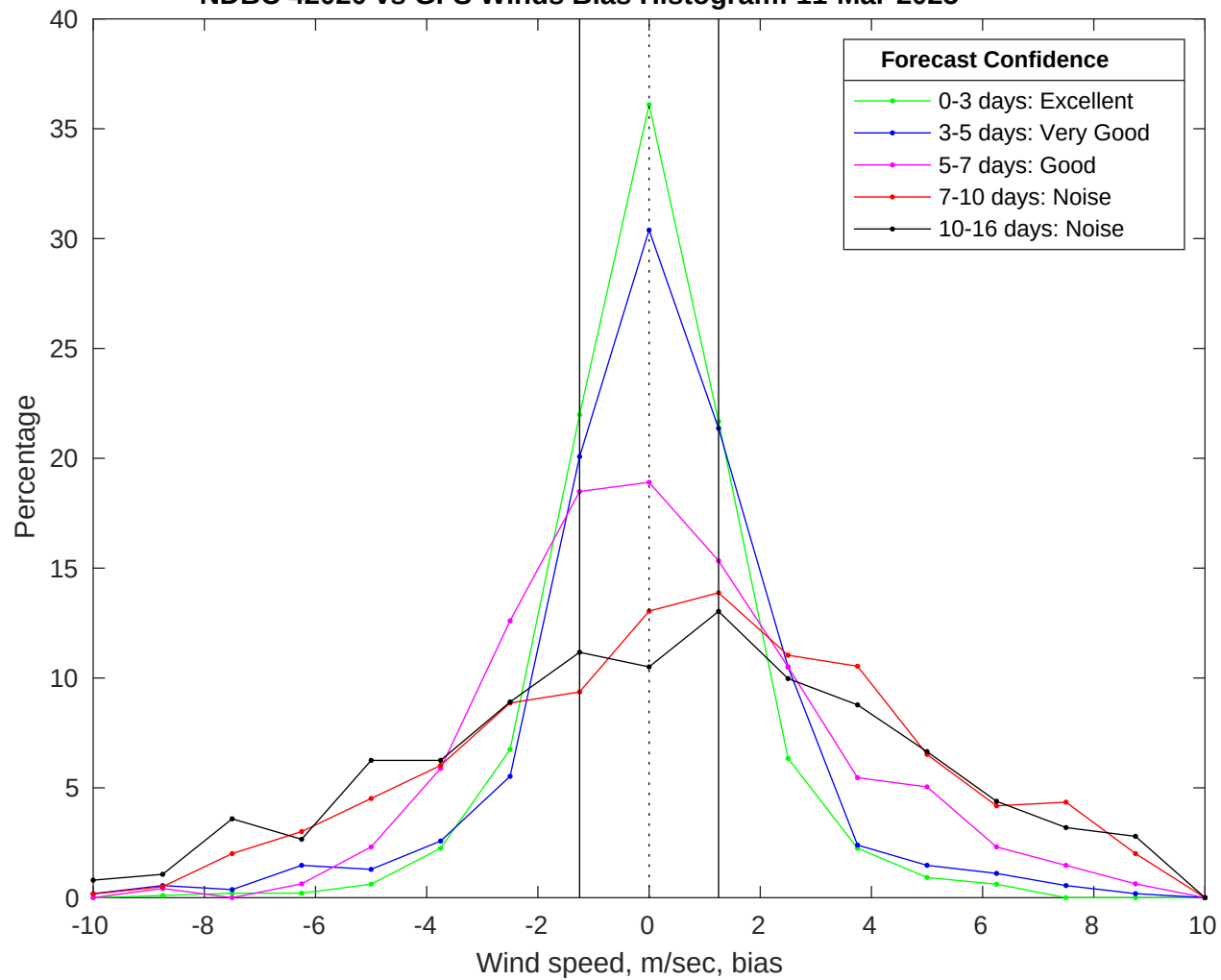
NDBC 42020 vs GFS Winds Bias Histogram: 11-Mar-2025
