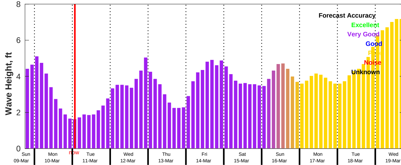
CMEMS Wave Forecast for NDBC 42020 from 09-Mar-2025 18:00:00 to 19-Mar-2025 18:00:00
