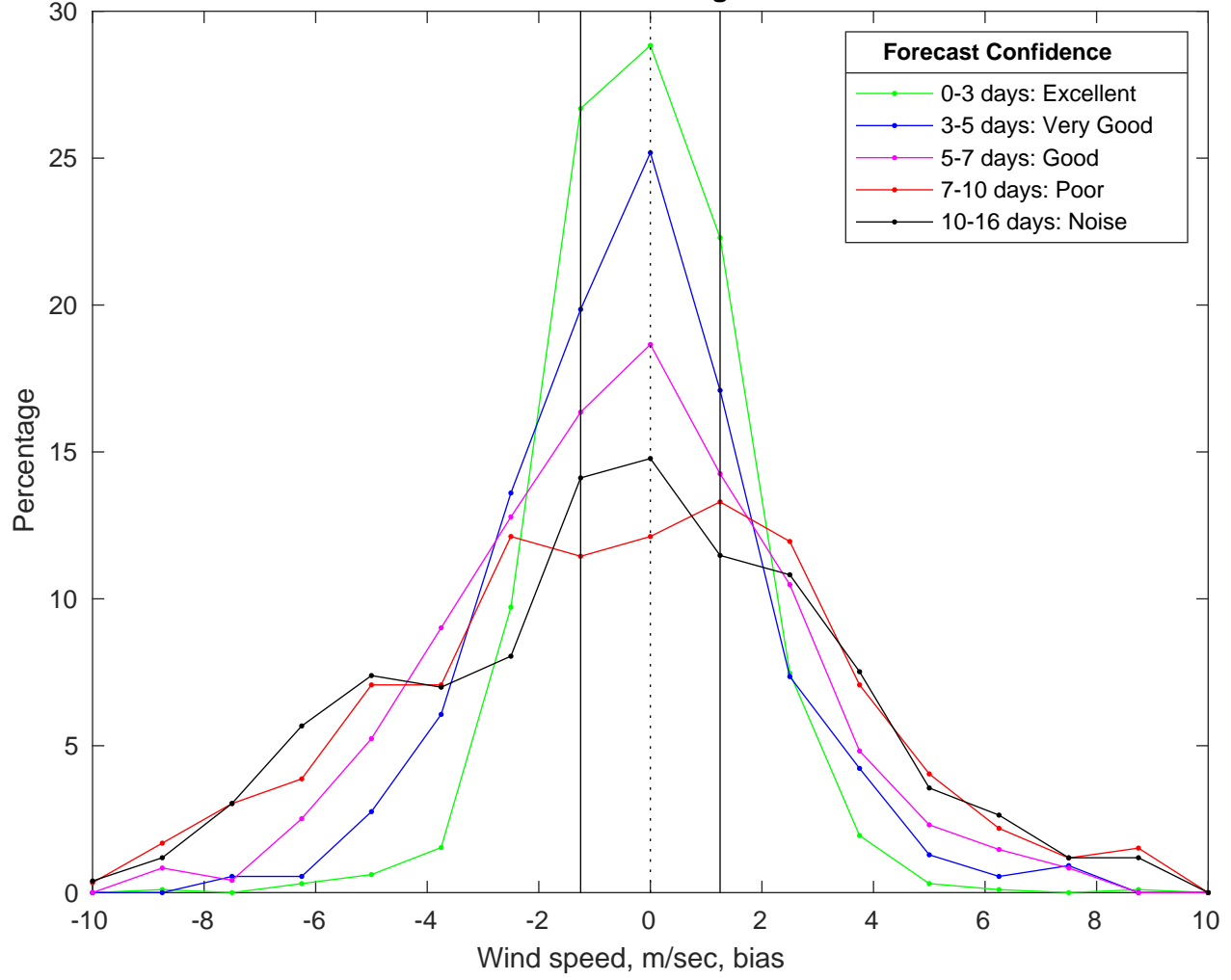
NDBC 42035 vs GFS Winds Bias Histogram: 11-Mar-2025
