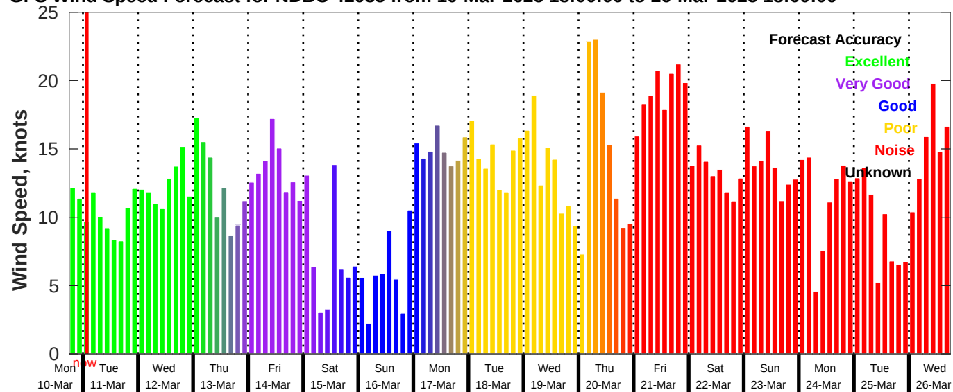
GFS Wind Speed Forecast for NDBC 42035 from 10-Mar-2025 18:00:00 to 26-Mar-2025 18:00:00
