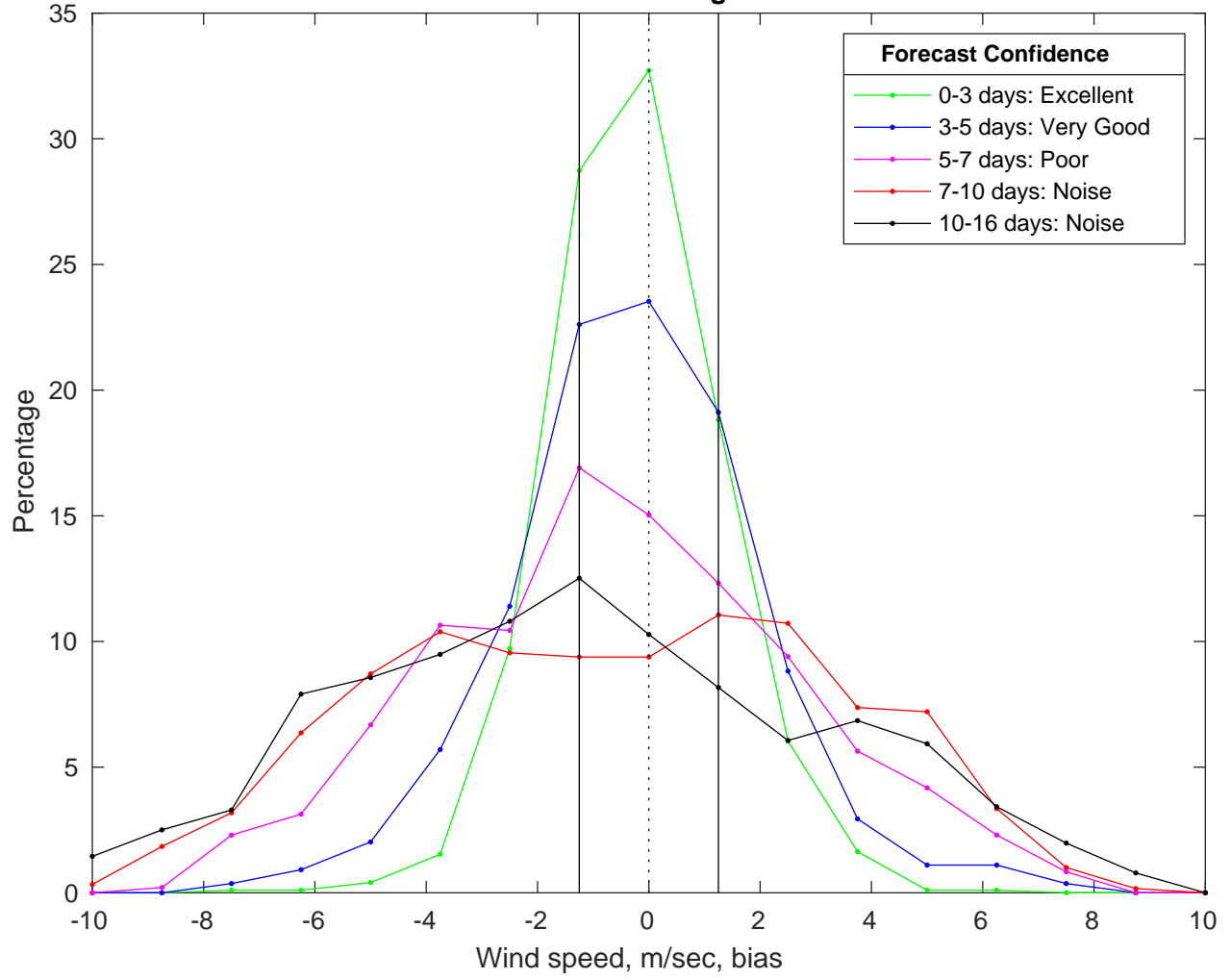
NDBC 42036 vs GFS Winds Bias Histogram: 11-Mar-2025
