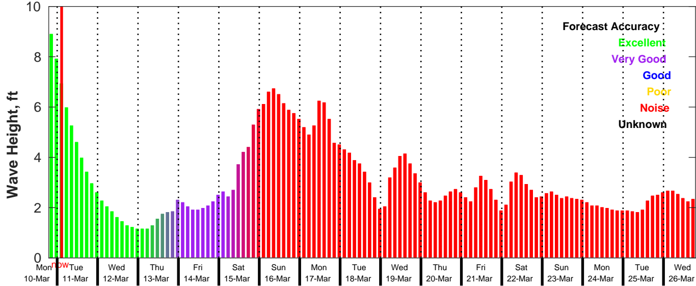
GFS Wave Forecast for NDBC 42036 from 10-Mar-2025 19:00:00 to 26-Mar-2025 19:00:00
