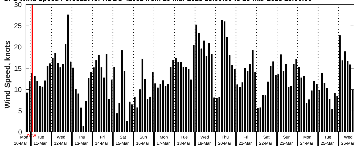
GFS Wind Speed Forecast for NDBC 42092 from 10-Mar-2025 18:00:00 to 26-Mar-2025 18:00:00
