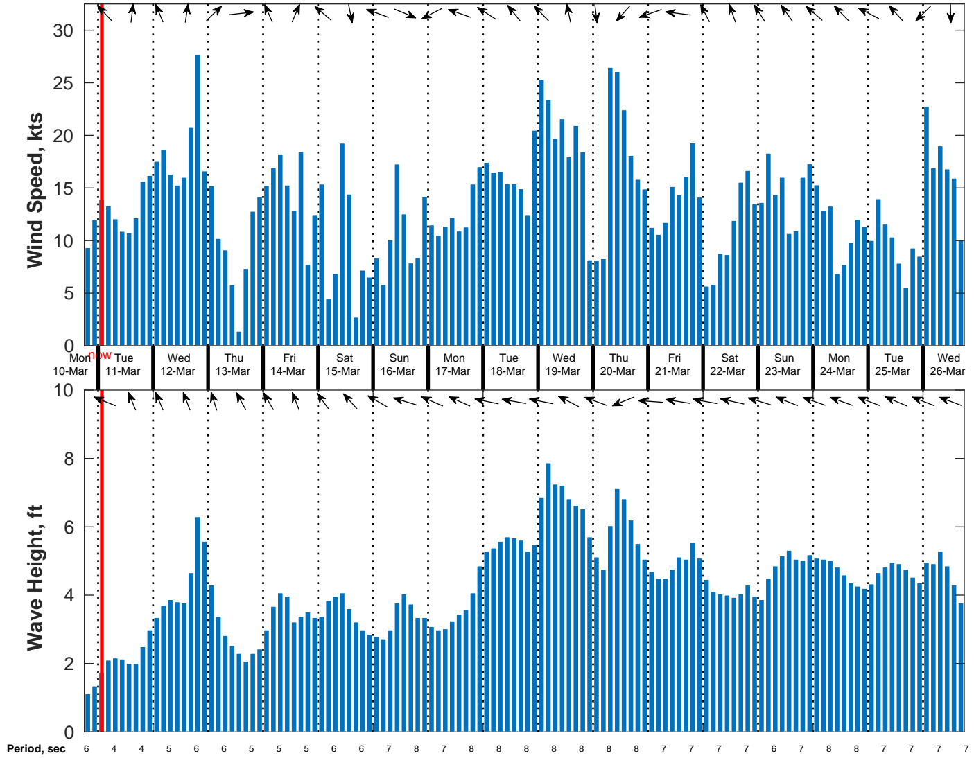
Wind & Wave Forecast for NDBC 42092 from 10-Mar-2025 18:00:00 to 26-Mar-2025 18:00:00
