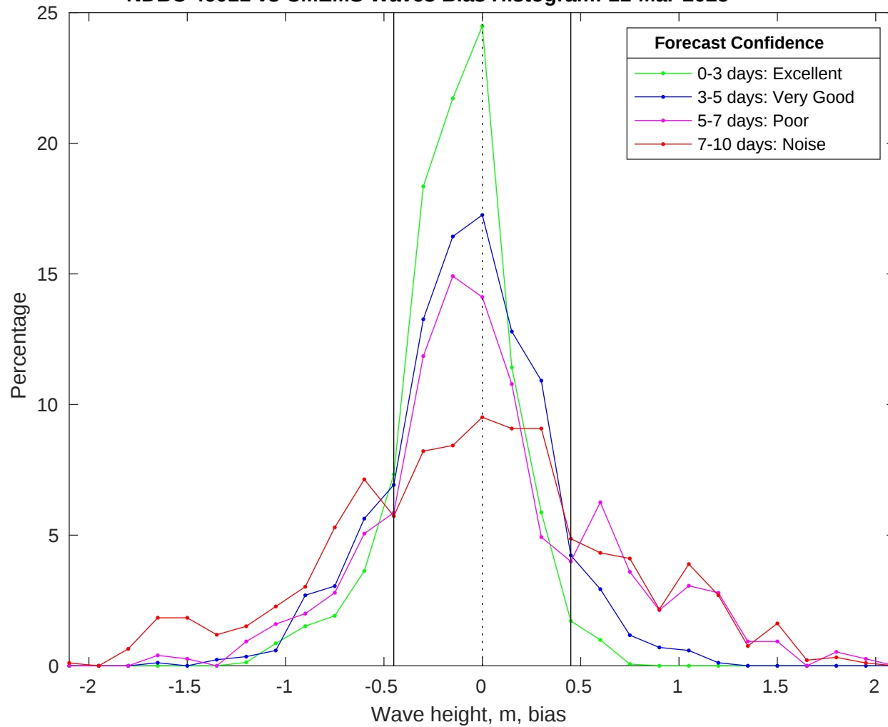
NDBC 46011 vs CMEMS Waves Bias Histogram: 11-Mar-2025
