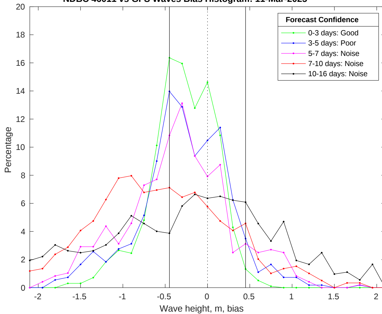
NDBC 46011 vs GFS Waves Bias Histogram: 11-Mar-2025
