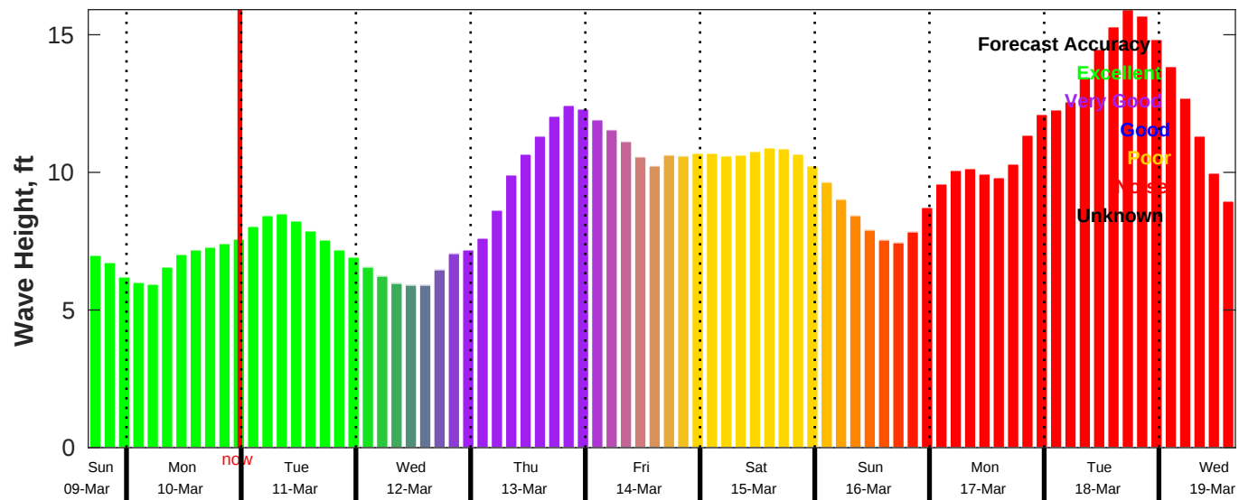
CMEMS Wave Forecast for NDBC 46011 from 09-Mar-2025 16:00:00 to 19-Mar-2025 16:00:00
