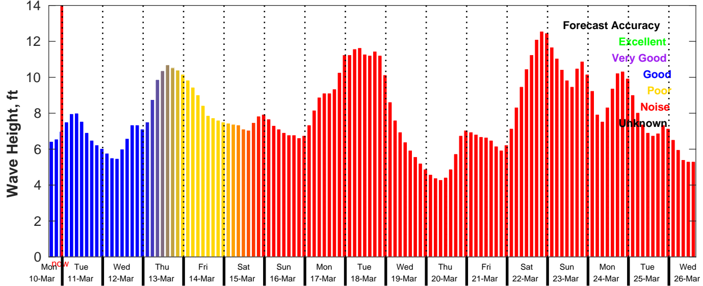
GFS Wave Forecast for NDBC 46011 from 10-Mar-2025 16:00:00 to 26-Mar-2025 16:00:00
