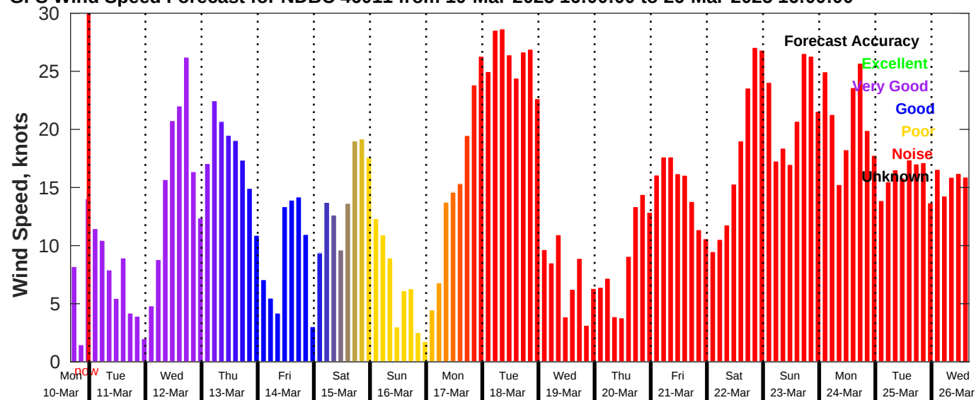
GFS Wind Speed Forecast for NDBC 46011 from 10-Mar-2025 16:00:00 to 26-Mar-2025 16:00:00
