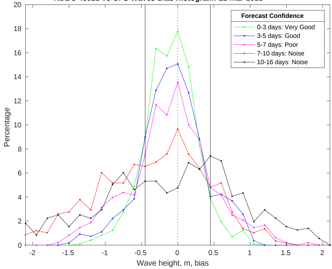
NDBC 46028 vs GFS Waves Bias Histogram: 11-Mar-2025
