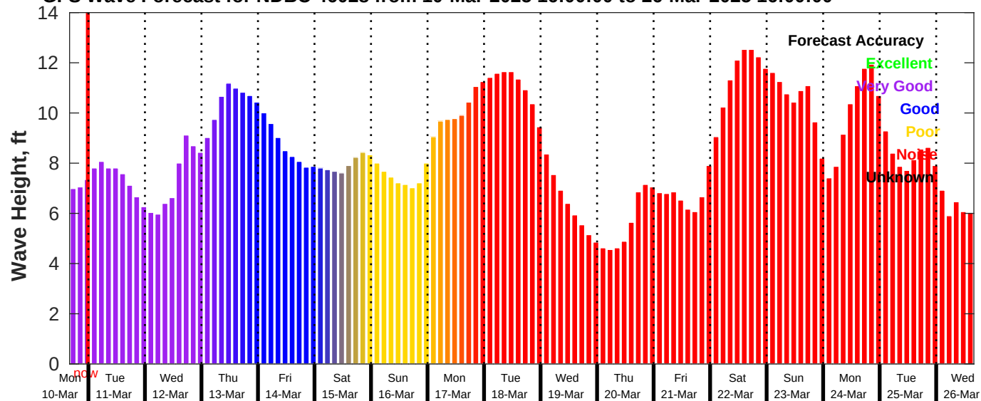
GFS Wave Forecast for NDBC 46028 from 10-Mar-2025 16:00:00 to 26-Mar-2025 16:00:00
