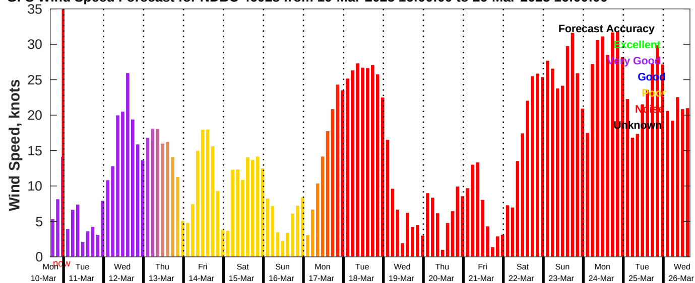
GFS Wind Speed Forecast for NDBC 46028 from 10-Mar-2025 16:00:00 to 26-Mar-2025 16:00:00
