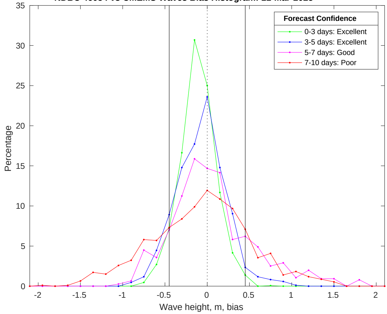
NDBC 46054 vs CMEMS Waves Bias Histogram: 11-Mar-2025
