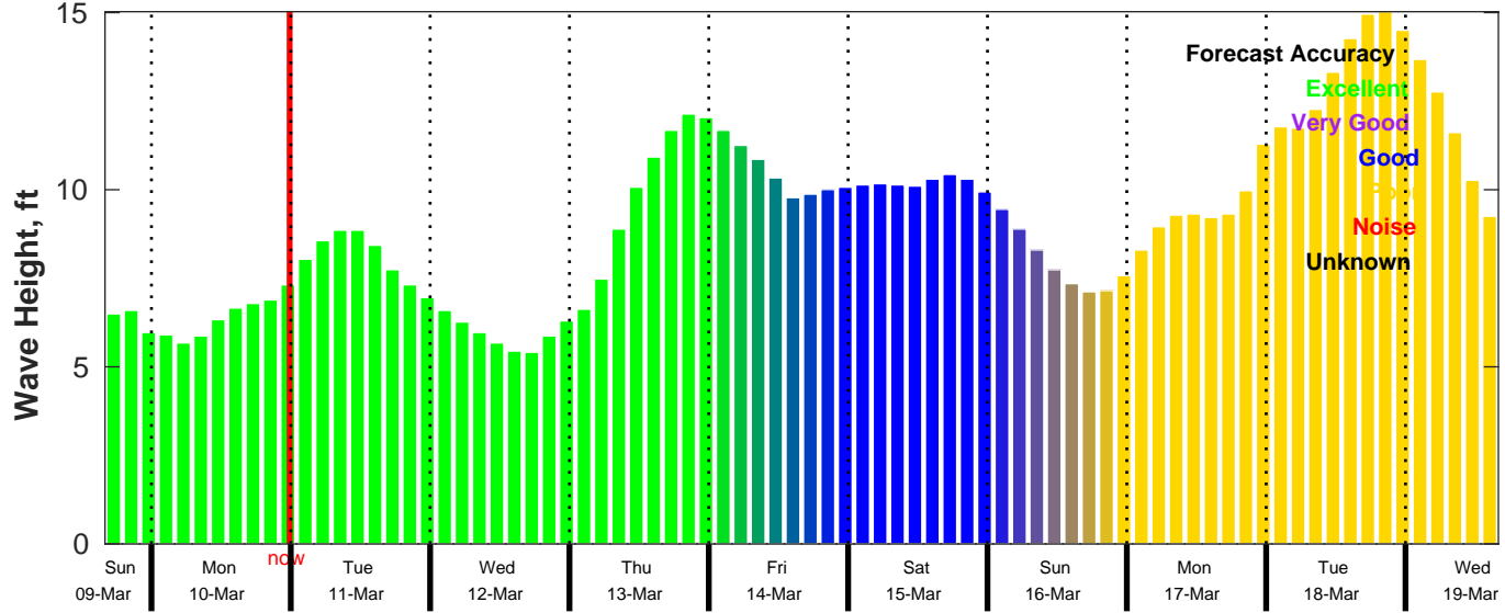
CMEMS Wave Forecast for NDBC 46054 from 09-Mar-2025 16:00:00 to 19-Mar-2025 16:00:00
