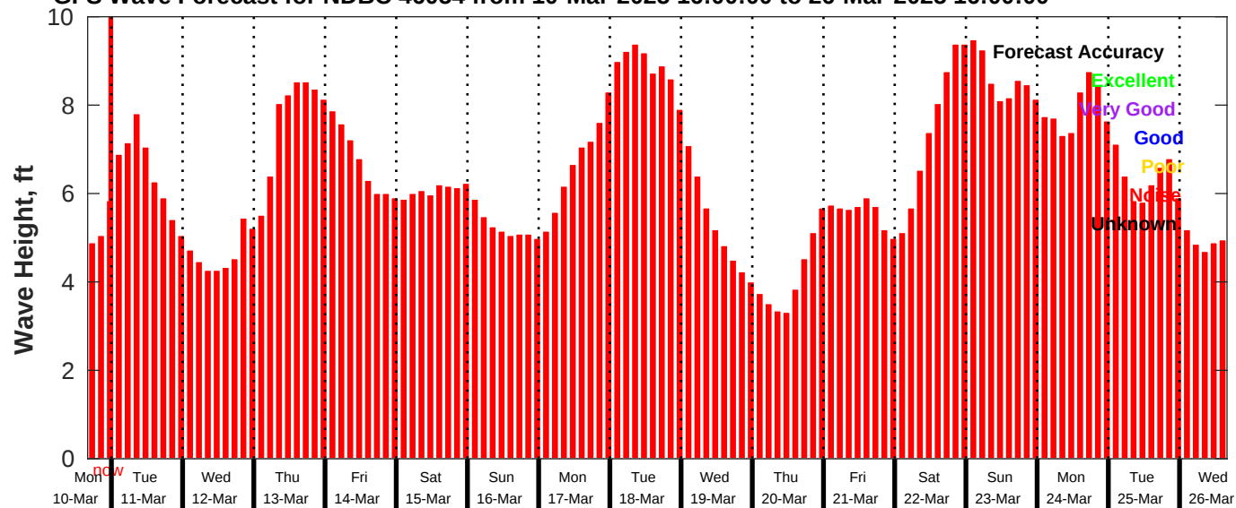
GFS Wave Forecast for NDBC 46054 from 10-Mar-2025 16:00:00 to 26-Mar-2025 16:00:00
