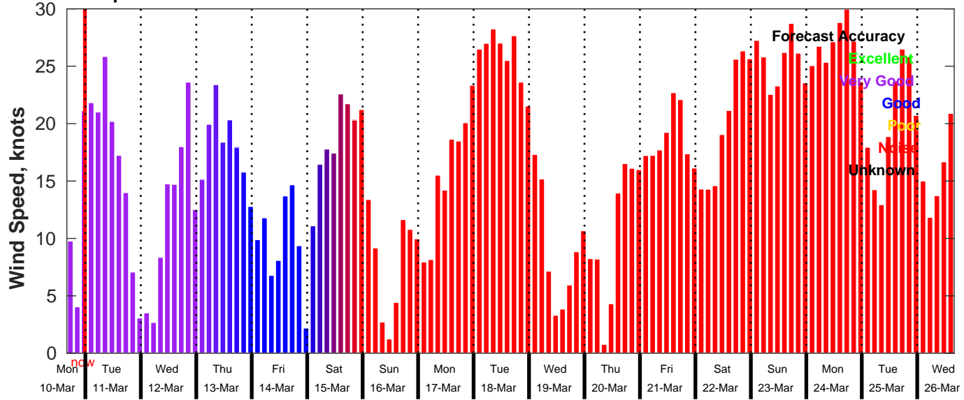
GFS Wind Speed Forecast for NDBC 46054 from 10-Mar-2025 16:00:00 to 26-Mar-2025 16:00:00
