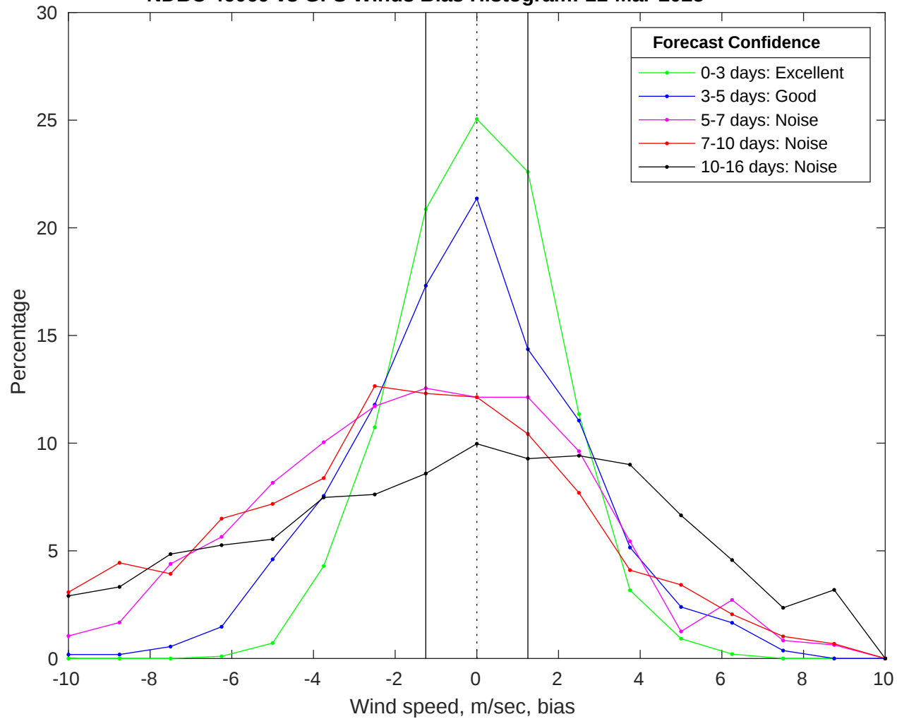
NDBC 46069 vs GFS Winds Bias Histogram: 11-Mar-2025
