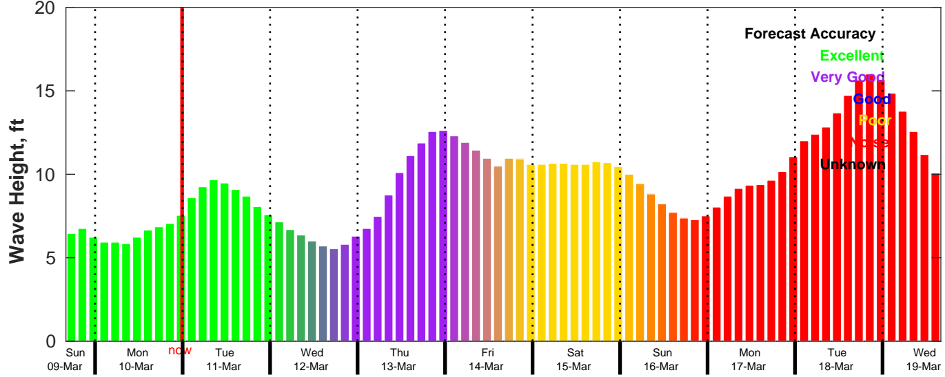
CMEMS Wave Forecast for NDBC 46069 from 09-Mar-2025 16:00:00 to 19-Mar-2025 16:00:00
