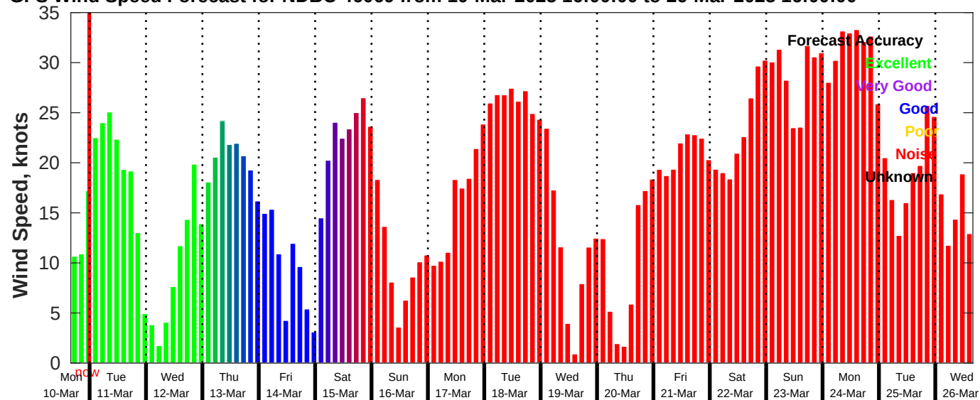
GFS Wind Speed Forecast for NDBC 46069 from 10-Mar-2025 16:00:00 to 26-Mar-2025 16:00:00
