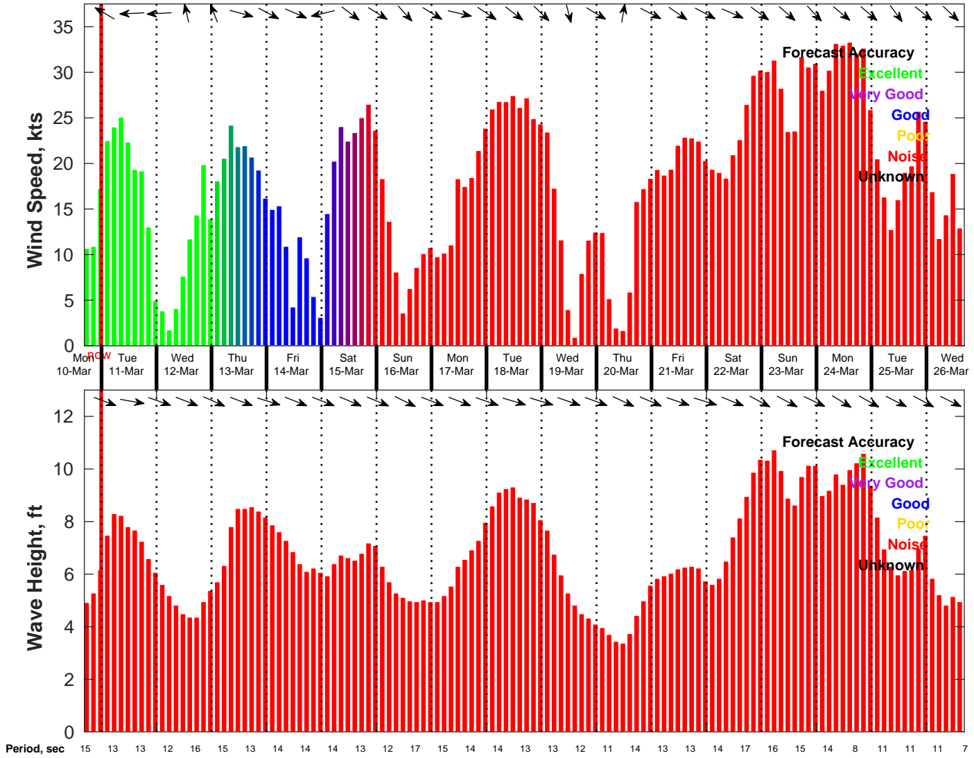
Wind & Wave Forecast for NDBC 46069 from 10-Mar-2025 16:00:00 to 26-Mar-2025 16:00:00
