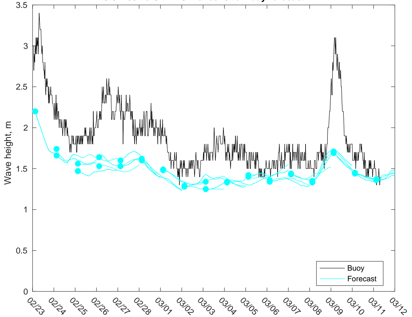
NDBC 51209 vs CMEMS Waves: 5 to 7 day forecast
