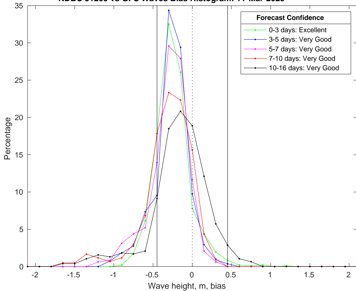
NDBC 51209 vs GFS Waves Bias Histogram: 11-Mar-2025
