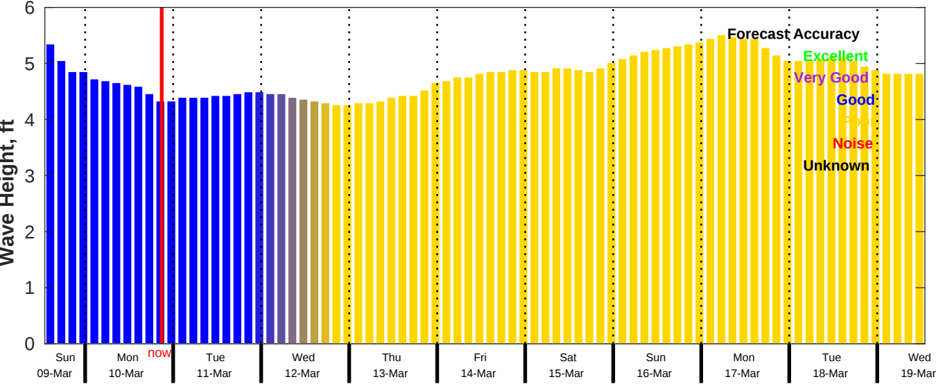
CMEMS Wave Forecast for NDBC 51209 from 09-Mar-2025 13:00:00 to 19-Mar-2025 13:00:00
