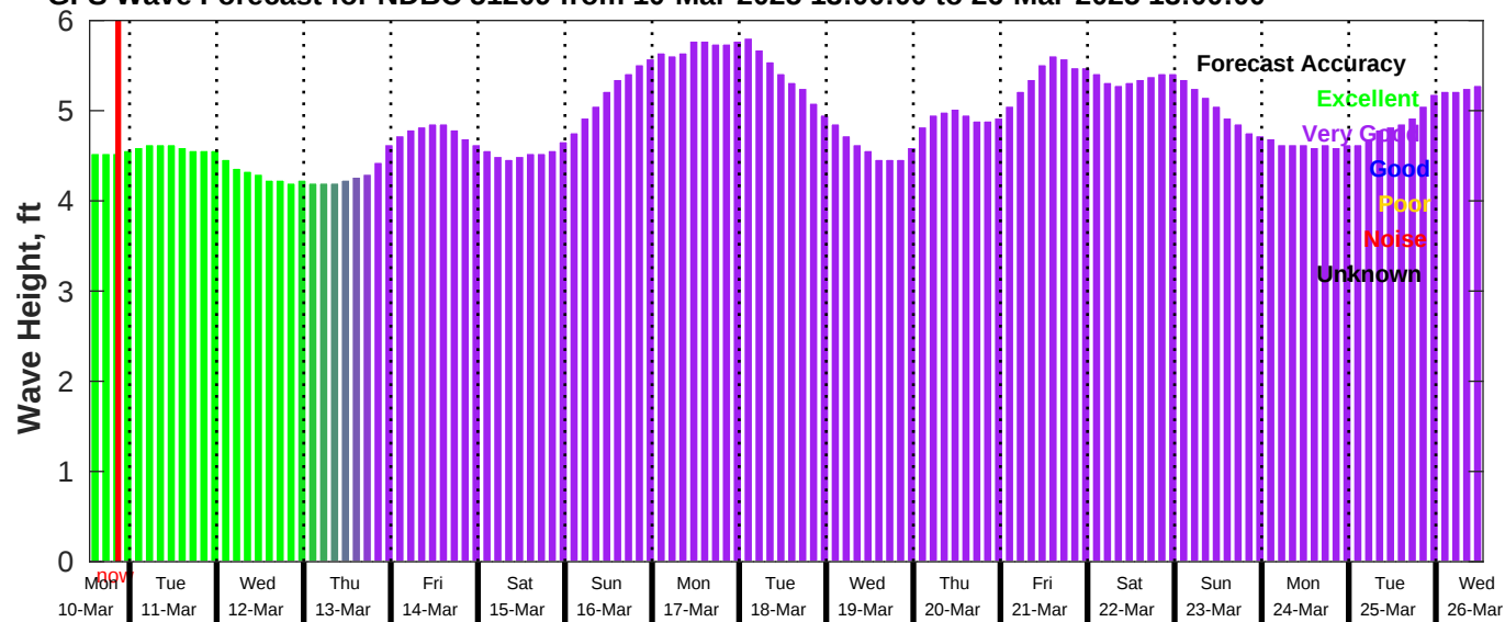
GFS Wave Forecast for NDBC 51209 from 10-Mar-2025 13:00:00 to 26-Mar-2025 13:00:00
