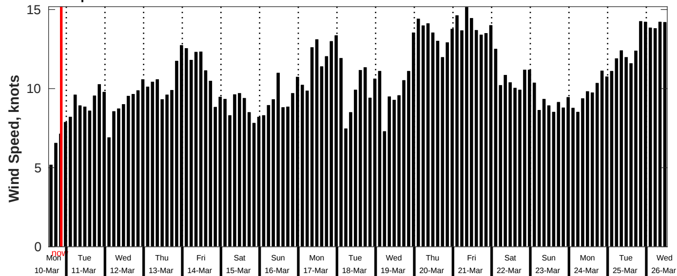
GFS Wind Speed Forecast for NDBC 51209 from 10-Mar-2025 13:00:00 to 26-Mar-2025 13:00:00
