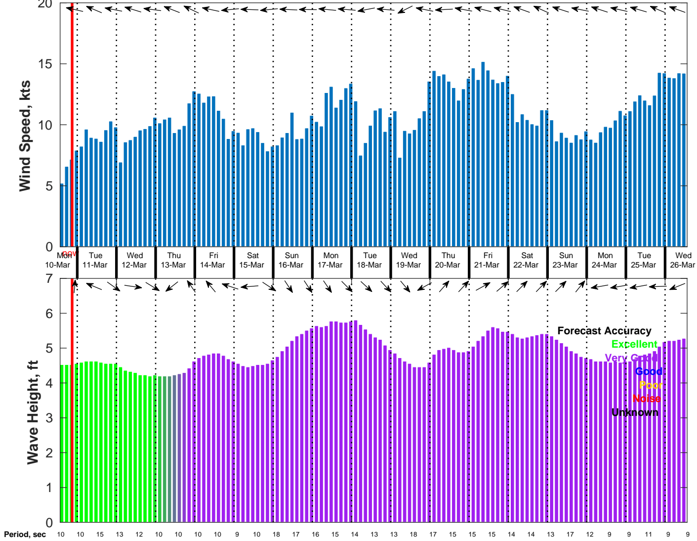
Wind & Wave Forecast for NDBC 51209 from 10-Mar-2025 13:00:00 to 26-Mar-2025 13:00:00
