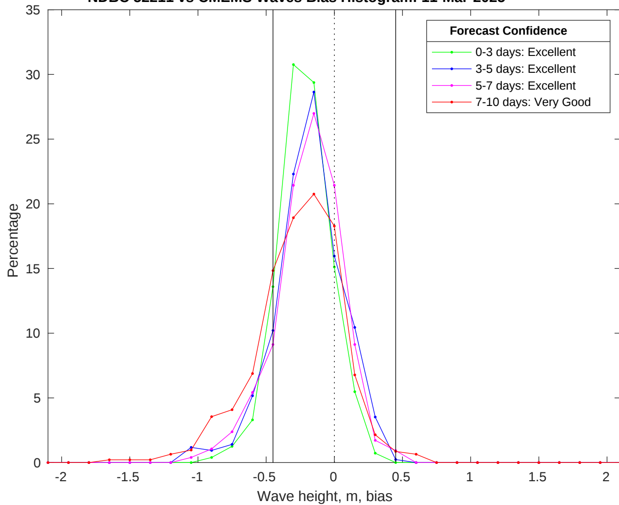
NDBC 52211 vs CMEMS Waves Bias Histogram: 11-Mar-2025
