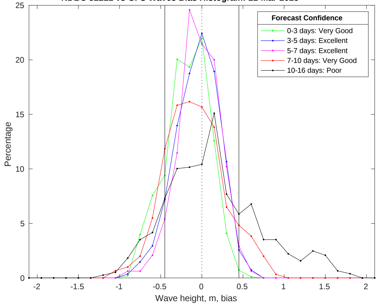
NDBC 52211 vs GFS Waves Bias Histogram: 11-Mar-2025
