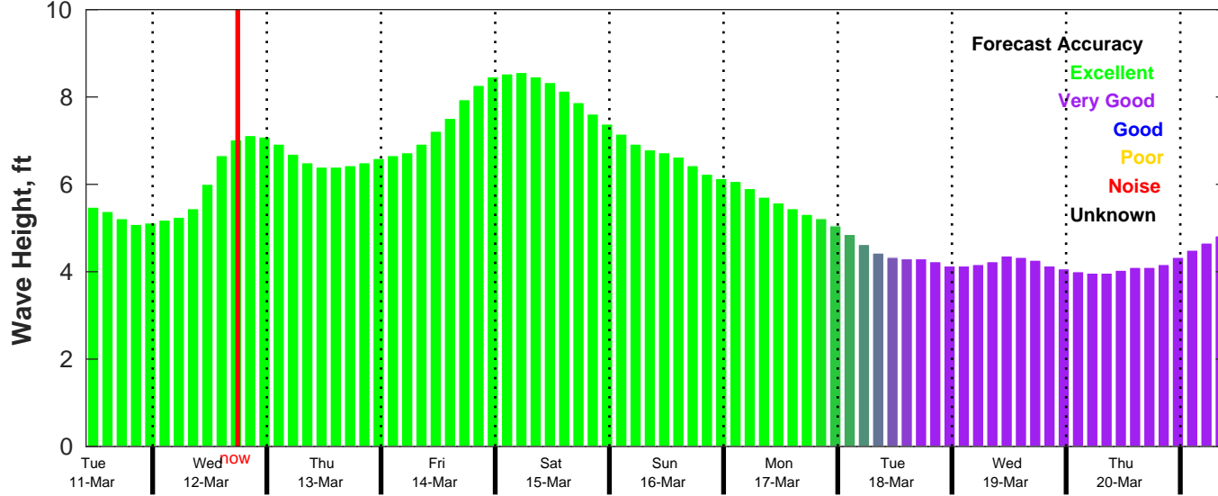
CMEMS Wave Forecast for NDBC 52211 from 10-Mar-2025 10:00:00 to 20-Mar-2025 10:00:00
