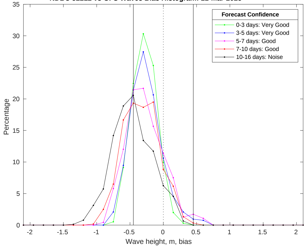
NDBC 52212 vs GFS Waves Bias Histogram: 11-Mar-2025
