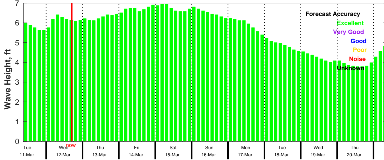
CMEMS Wave Forecast for NDBC 52212 from 10-Mar-2025 09:00:00 to 20-Mar-2025 09:00:00
