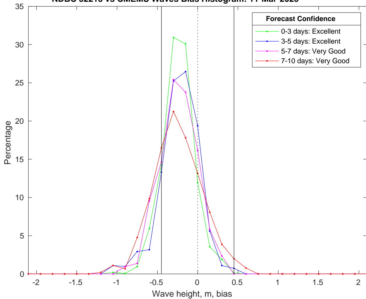
NDBC 52213 vs CMEMS Waves Bias Histogram: 11-Mar-2025
