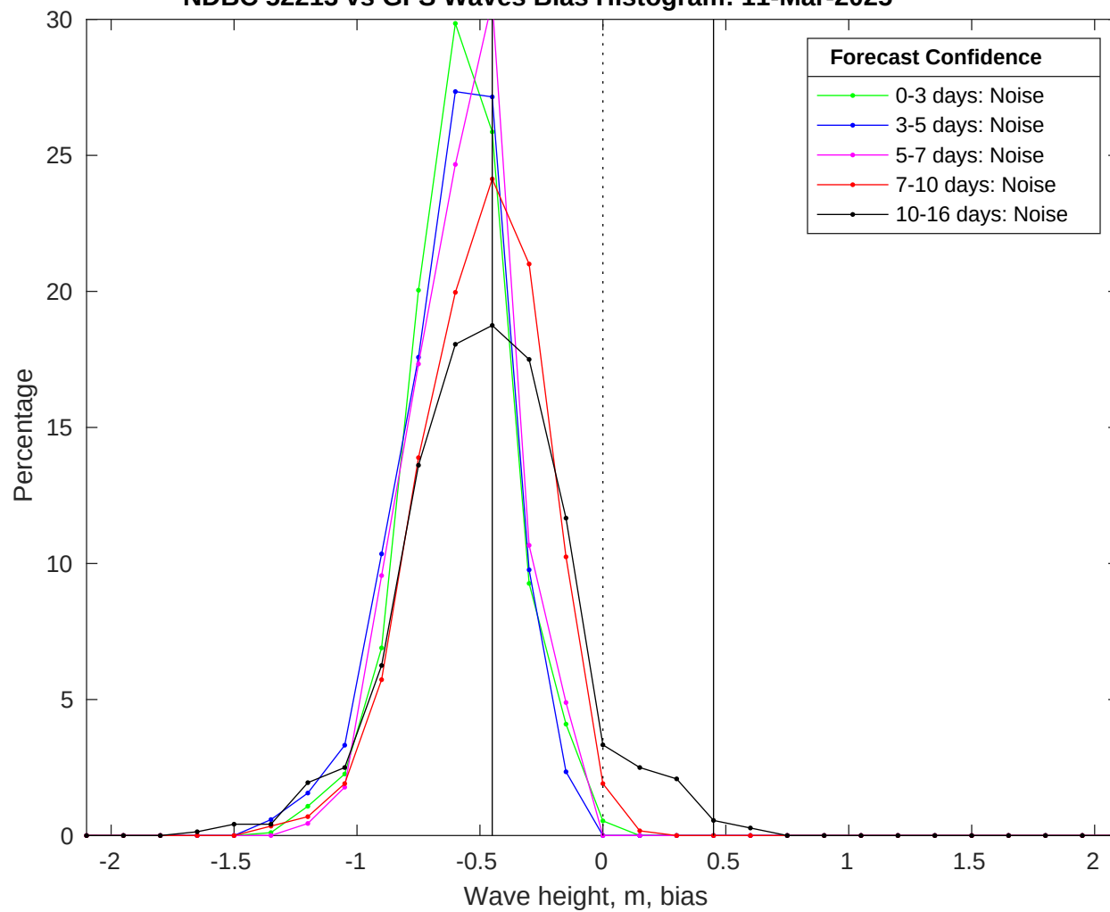
NDBC 52213 vs GFS Waves Bias Histogram: 11-Mar-2025
