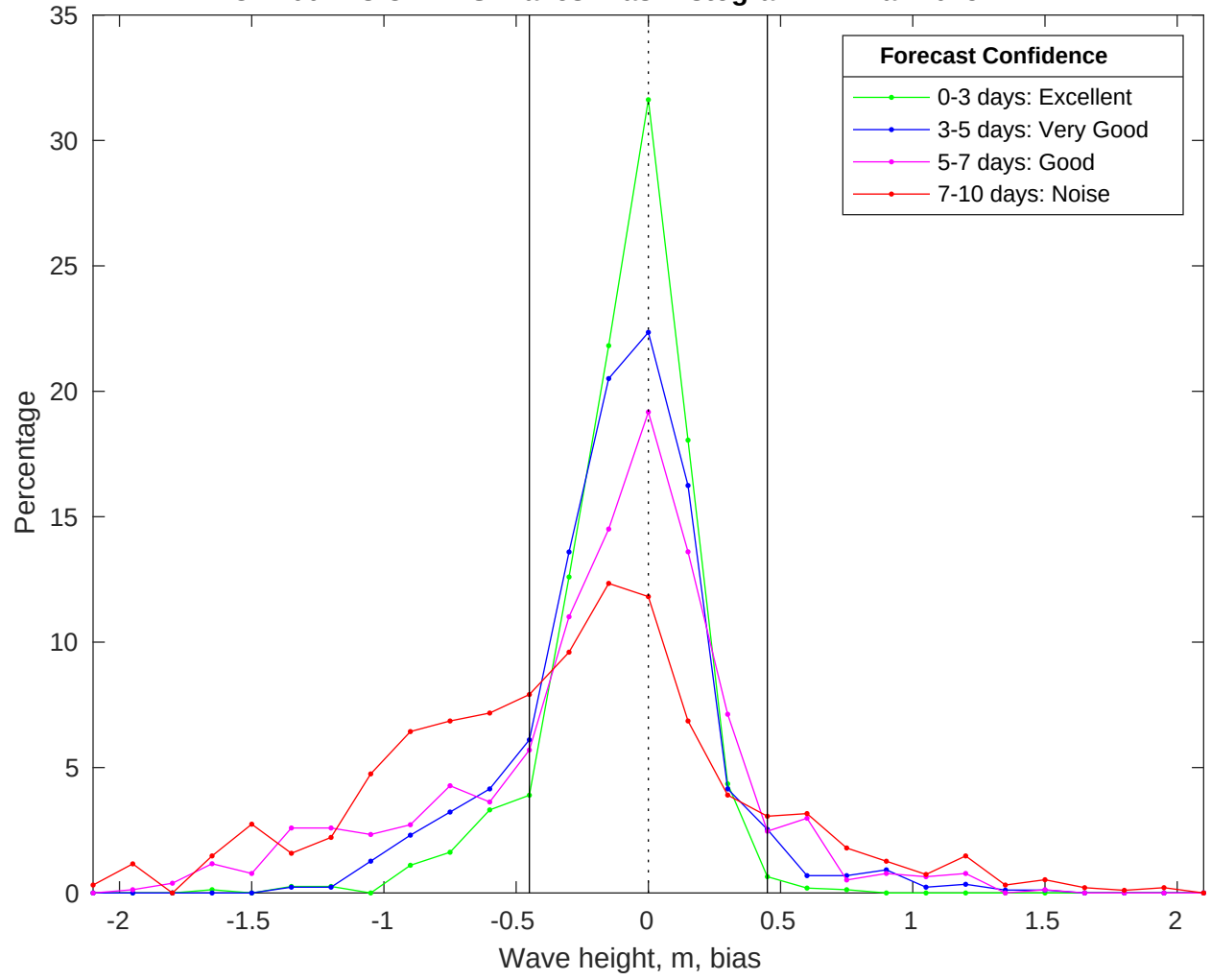
NDBC 41004 vs CMEMS Waves Bias Histogram: 12-Mar-2025
