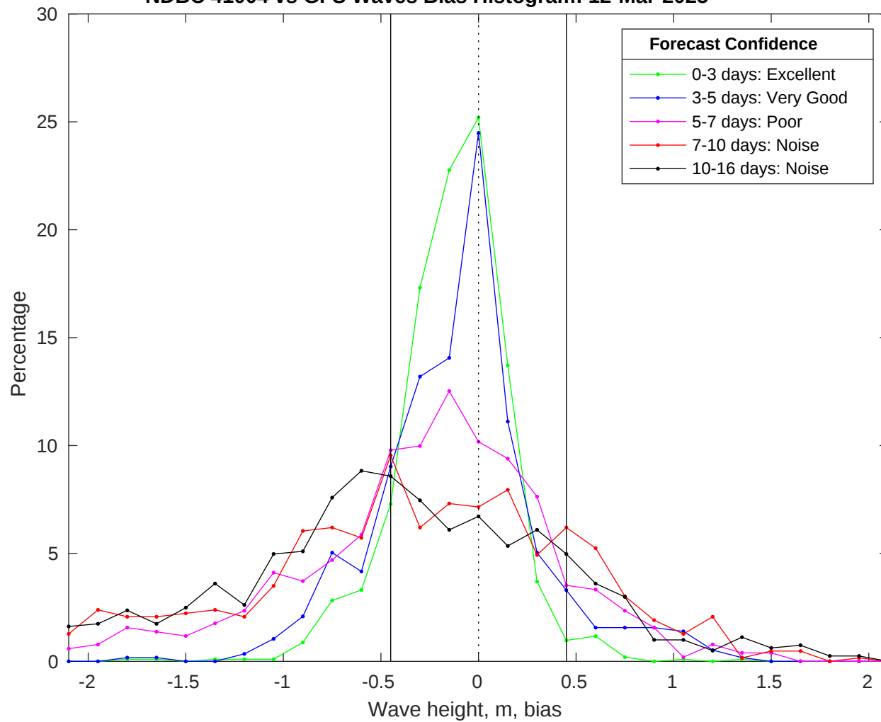
NDBC 41004 vs GFS Waves Bias Histogram: 12-Mar-2025
