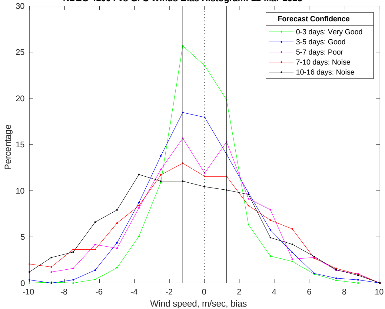
NDBC 41004 vs GFS Winds Bias Histogram: 12-Mar-2025
