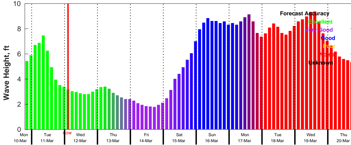
CMEMS Wave Forecast for NDBC 41004 from 10-Mar-2025 19:00:00 to 20-Mar-2025 19:00:00
